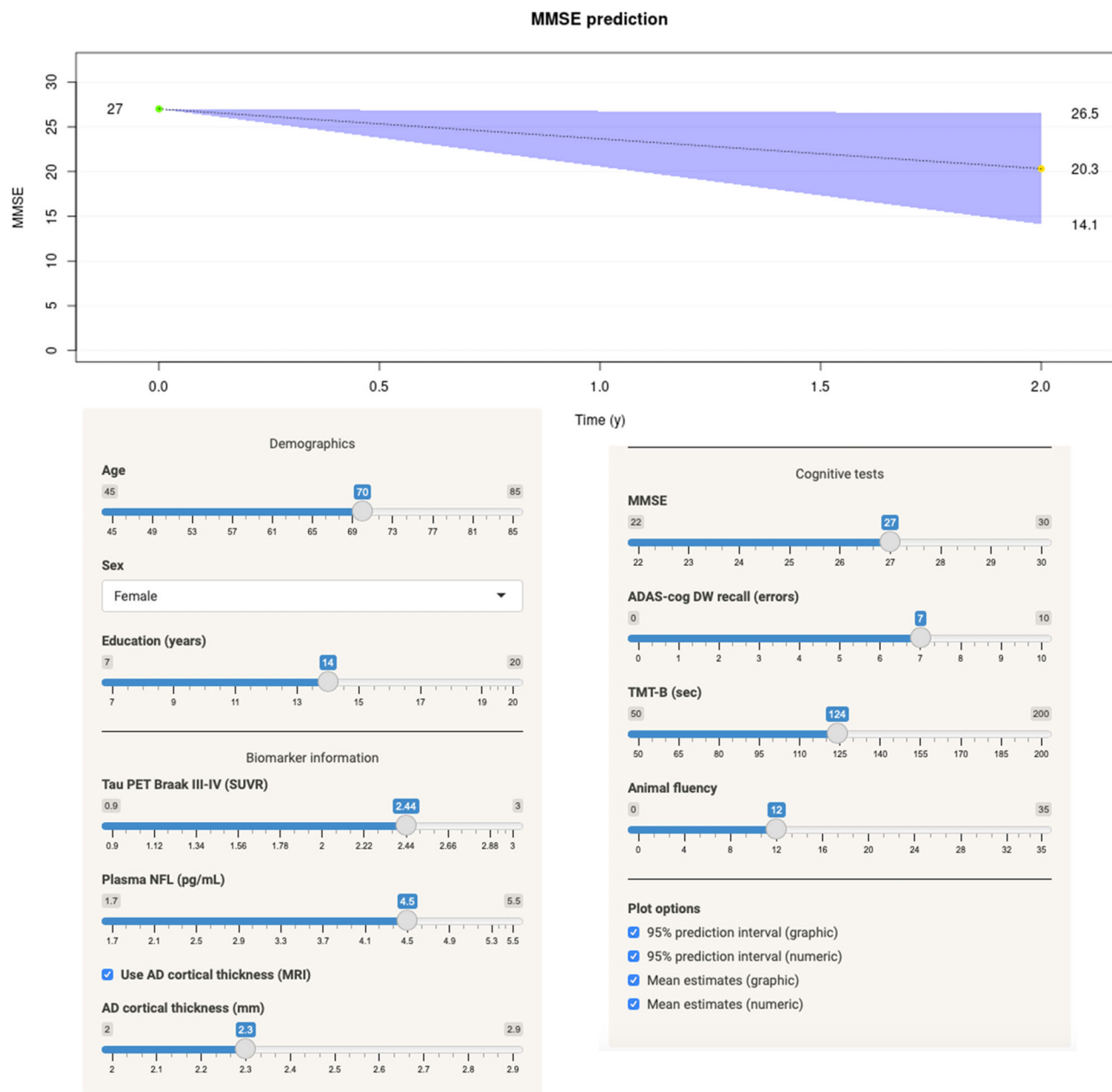
FIGURE 3 Prediction algorithm for cognitive decline. Example of the implementation of the regression models at https://brainapps.shinyapps.io/PredictMMSE/ . At this website it is possible to enter basic demographic data (age, sex, and education), biomarker data (tau-PET temporal Region-of-interest (ROI) Standardized Uptake Value Ratio (SUVR) and plasma Neurofilament Light (NfL) [pg/mL]) as well as raw cognitive test scores (Mini-Mental State Examination (MMSE), Alzheimer's Disease Assessment Scale (ADAS) delayed recall, Trail-making test-B (TMT-B), and animal fluency). The example shows the predicted individual change in cognition for a 70-year-old woman who has 14 years of education, a pathological tau-PET (2.44 SUVR), a plasma NfL of 4.5 pg/mL, and a cortical thickness of 2.3 mm (please note that entering cortical thickness is optional). She has a baseline MMSE score of 27, scores seven errors on a 10-word delayed-recall test, completes the Trail-Making Test B in 124 s, and names 12 animals in 1 min
