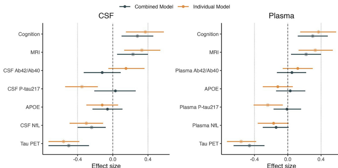
FIGURE 1 Prediction of cognitive decline using biomarkers individually or in combination. The figure shows the effect sizes for each biomarker in predicting future cognitive decline either alone (orange bars, on top) or in a combined model (black bars, below). Significant biomarkers are represented with a star. The model using cerebrospinal fluid (CSF) biomarkers is shown in the left panel and the model using plasma biomarkers in the right panel. Bars represent 95% confidence intervals
