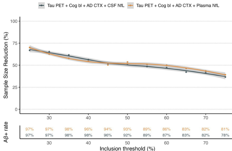
FIGURE 2 Enrichment for clinical trials using the parsimonious model biomarkers. The top panel of the graph shows the effect on group size needed to include in a clinical trial to retain statistical power when enriching for pathological values for the tau-PET (positron emission tomography), baseline cognition, cortical thickness, and neurofilament light (NfL) biomarkers (cerebrospinal fluid [CSF] NfL in black; plasma NfL in orange). The bottom panel shows the rate of amyloid beta ( A\beta ) positivity with the different inclusion thresholds (CSF in black; plasma in orange)
